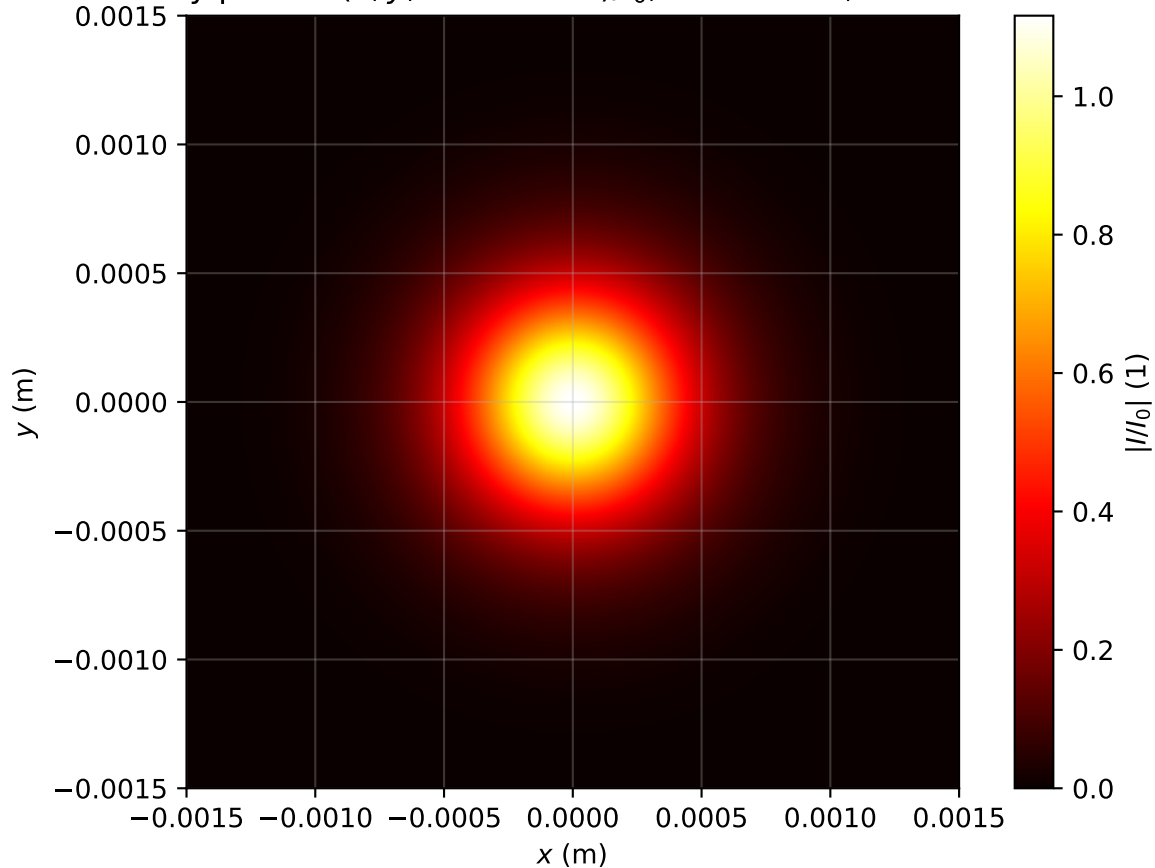
Intensity profile I(x, y, z = 1.115m)/I_0 , P_{in}=0.6P_{cr} , artificial time
